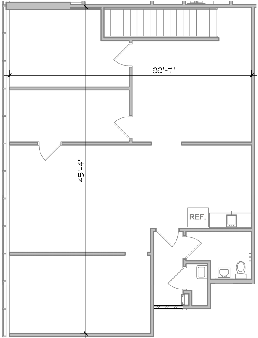
2 UPPER LEVEL 9053 1,443 R.S.F. 1/8" = 1'-0"
