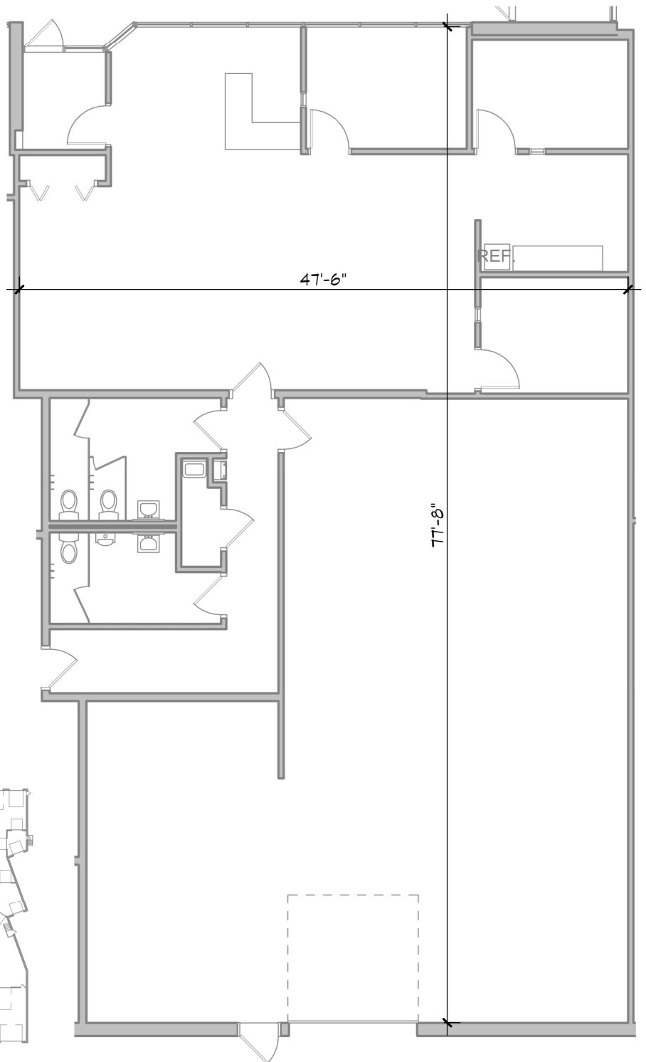
1 SUITE 9059 PLAN 9059 3/32" = 1'-0"
