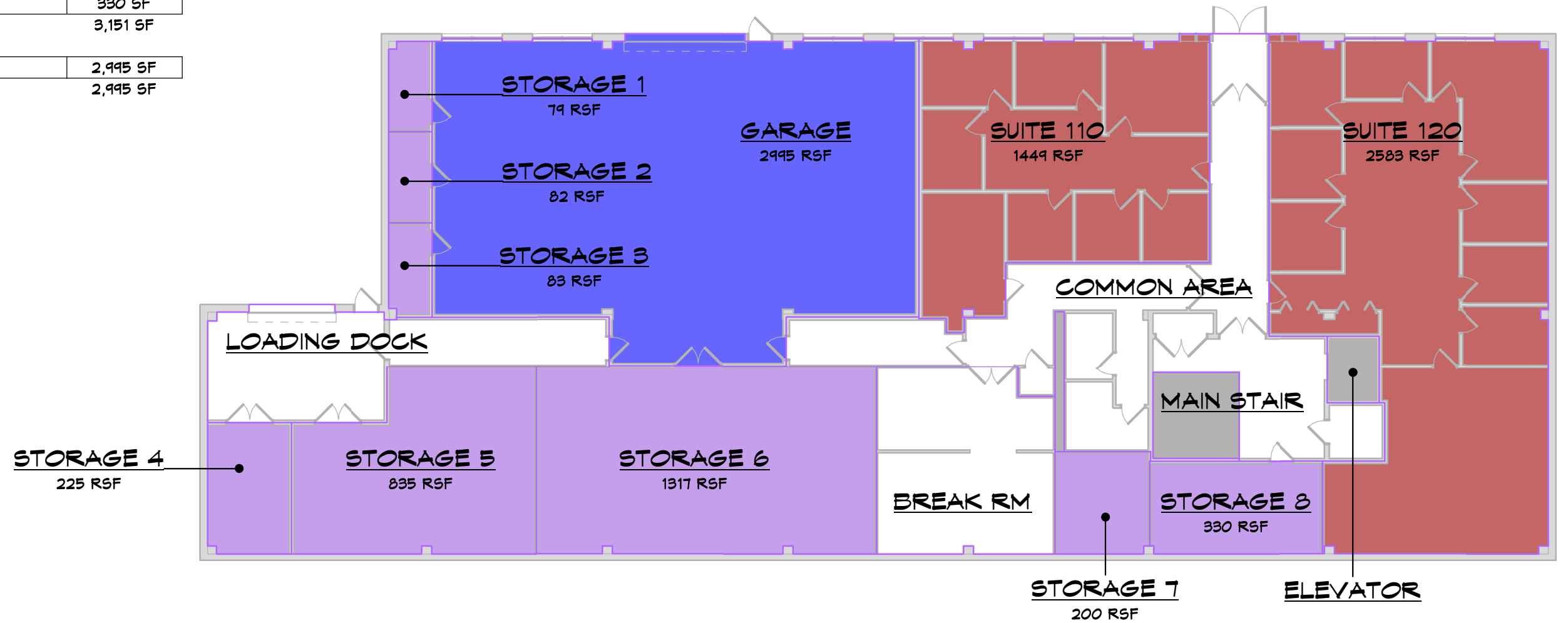
1 LEVEL 1 RENTABLE AREA PLAN L1 1/16" = 1'-0"
