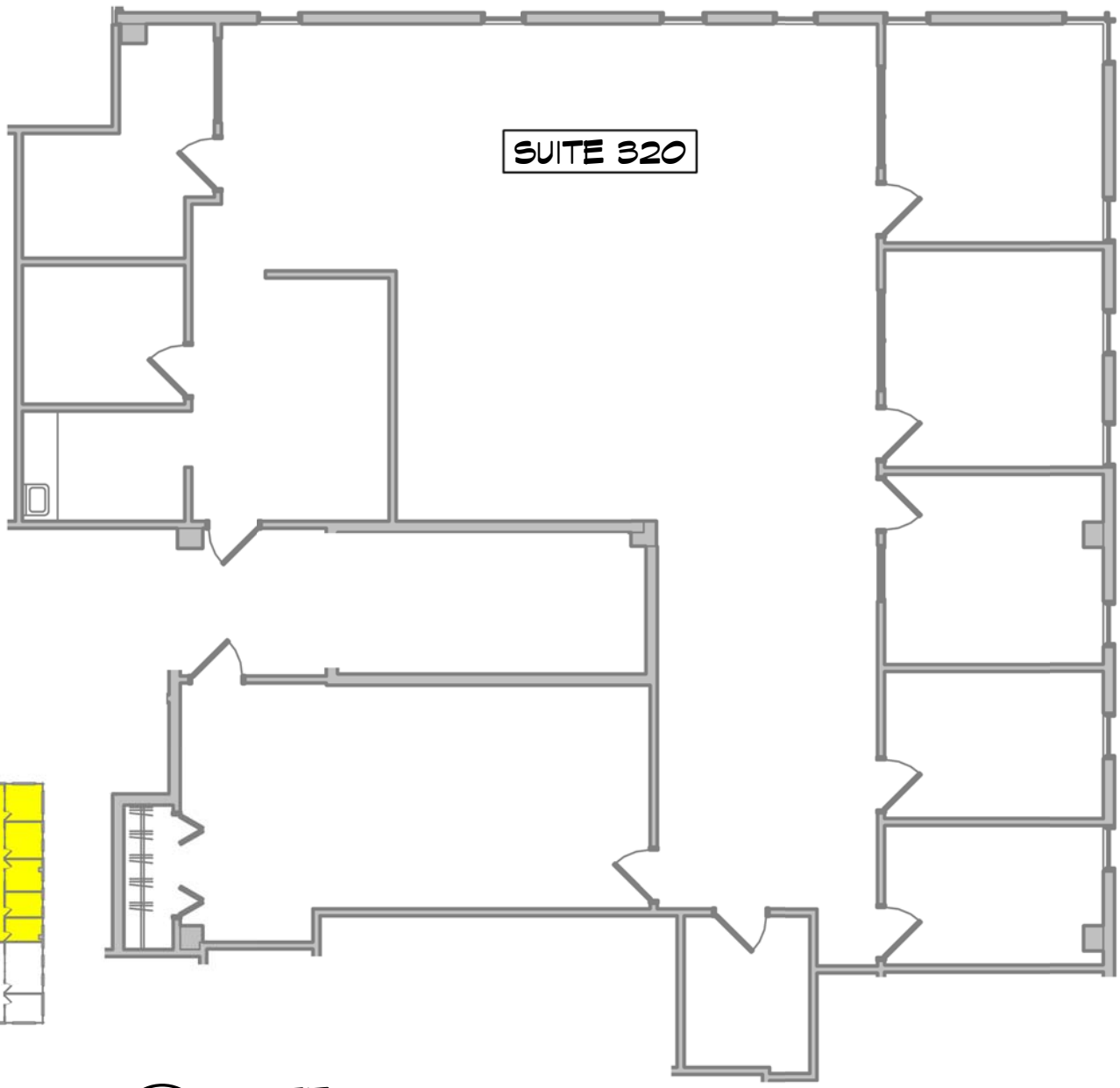
SUITE 320 1" = 10'-0"
